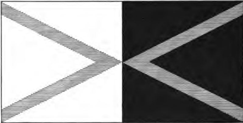
Fig. 63. — Illustrating brightness-contrast.
